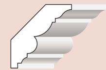
BMCR 602 6" W x 4 5/16" H x 4 3/16" D
