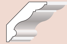
BMCR 901 9 1/2" W x 6 5/8" H x 6 7/8" D
