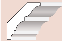
BMCR 405 4" W x 3" H x 2 3/4" D
