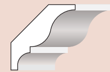
BMCR 603 6 1/8" W x 4 5/16" H x 4 3/16" D
