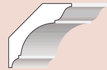
BMCR 801 8 1/8" W x 5 3/4" H x 5 3/4" D
