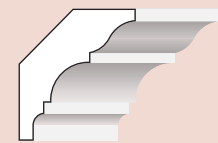
BMCR 502 5" W x 3 3/4" H x 3 3/8" D
