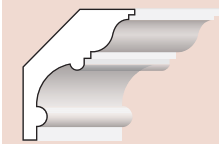
BMCR 604 6 1/16" W x 4 9/16" H x 4" D
